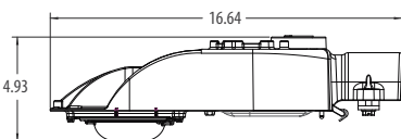
R3/R5 Optic
